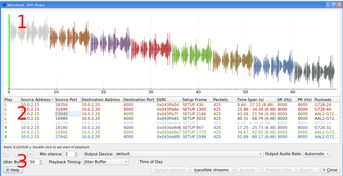
Figure 112. RTP Player window
